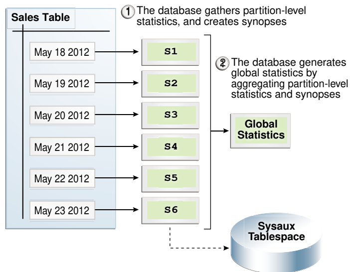
Figure 13-2 Aggregating Statistics
