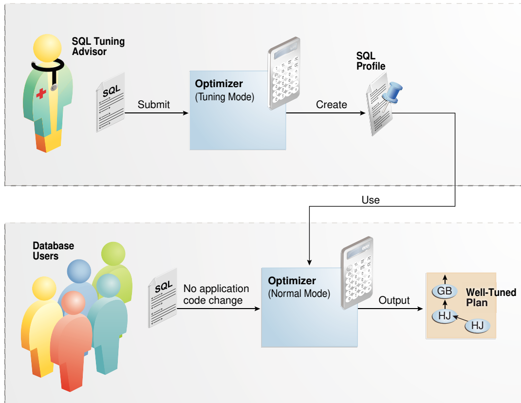
Figure 24-4 SQL Profile
