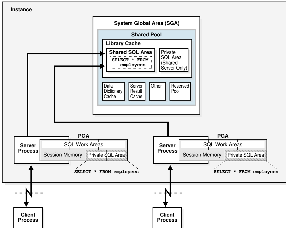
Figure 20-2 Cursor Sharing
