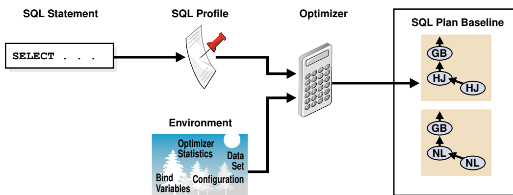
Figure 26-1 SQL Profile
