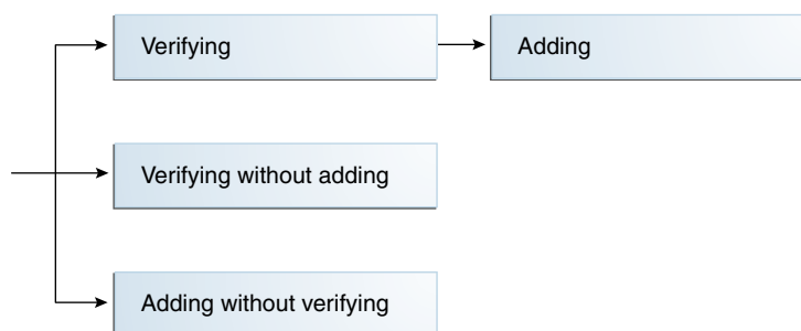
Figure 27-4 Plan Evolution
