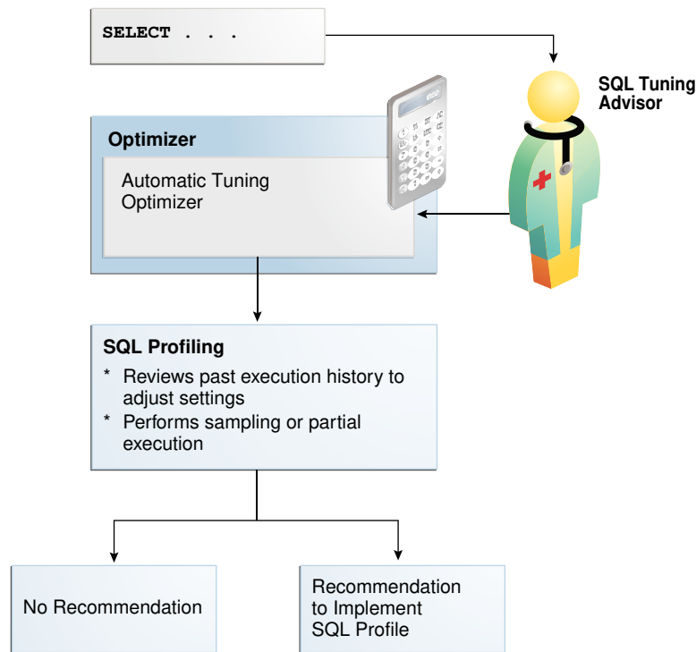
Figure 24-5 SQL Profiling
