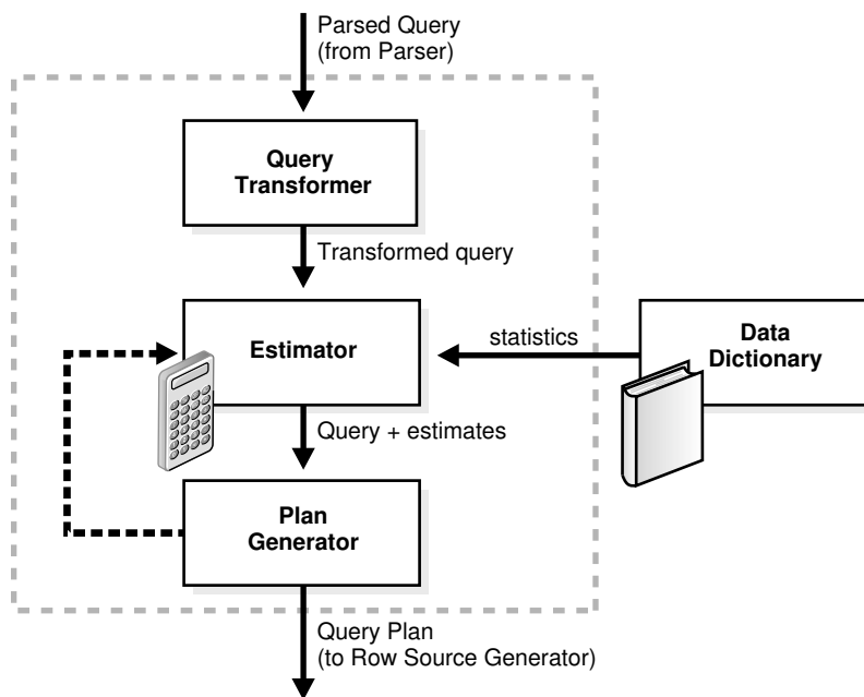
Figure 4-2 Optimizer Components
