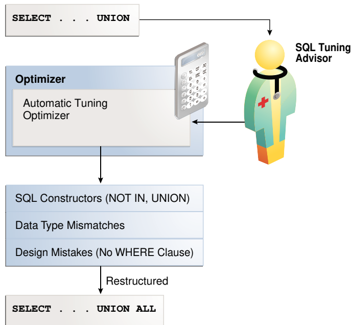
Figure 24-8 Structural Analysis
