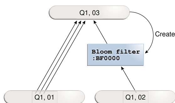
Figure 9-8 Bloom Filter
