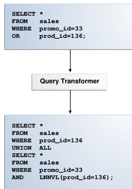
Figure 4-3 Query Transformer
